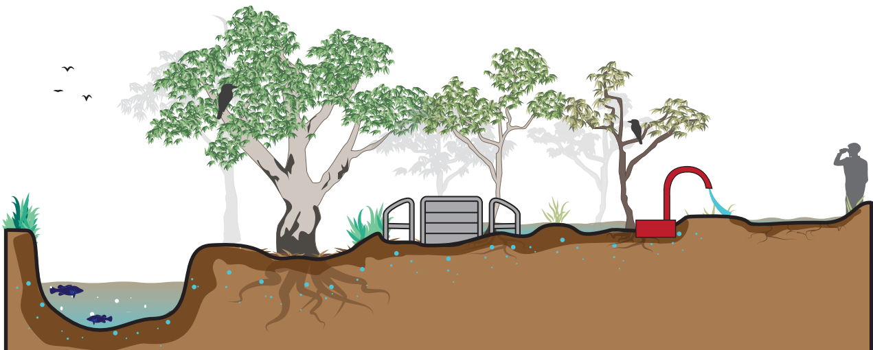
Scenario 3: If the floodplain is too dry, we can use a temporary pump to get environmental water onto the floodplain and close the regulators to hold the water there for as long as needed, before returning the water to the river.
